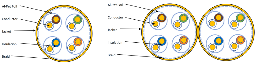
Single cable
